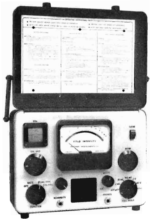
FIM-21 Field Intensity Meter
