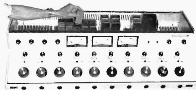
IC-10, Showing Plug-In Modules
