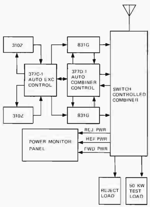
831H Block Diagram
