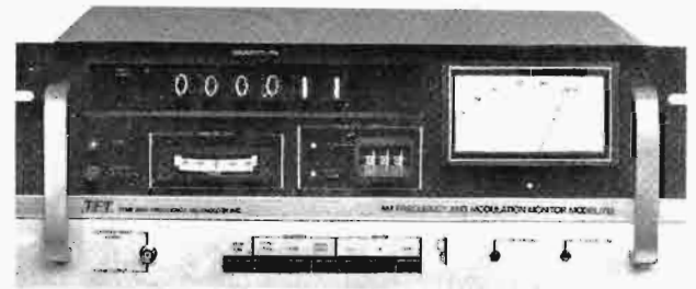
TFT 713 AM Frequency/Modulation Monitor
